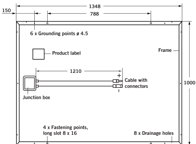
Abb. 3: External dimensions (in mm) and components for Q.PEAK S
