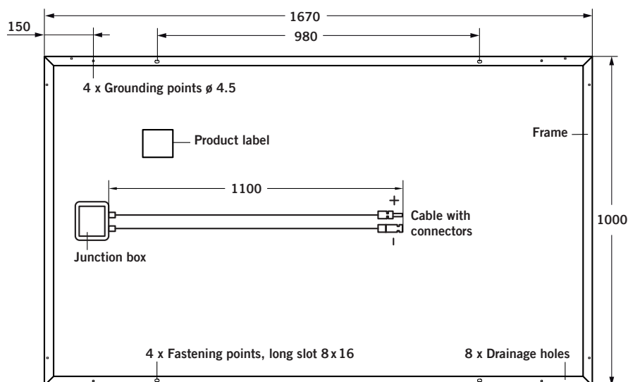
Abb. 1: External dimensions (in mm) and components for Q.PRO-G2 (up to Version 03), Q.PEAK (up to Version 04), Q.PEAK BLK (up to Version 02)
