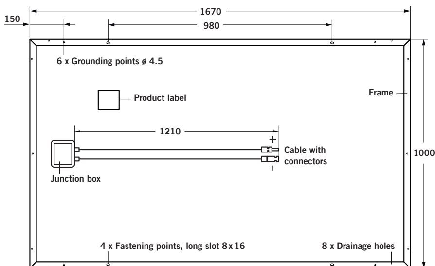
Abb. 2: External dimensions (in mm) and components for Q.PRO-G2 (Version 04 & up), Q.PEAK (Version 05 & up), Q.PEAK BLK (Version 03 & up), Q.PEAK BLK-G2, Q.PEAK-G2
